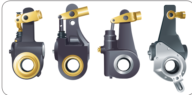
Four types of automatic slack adjusters.
